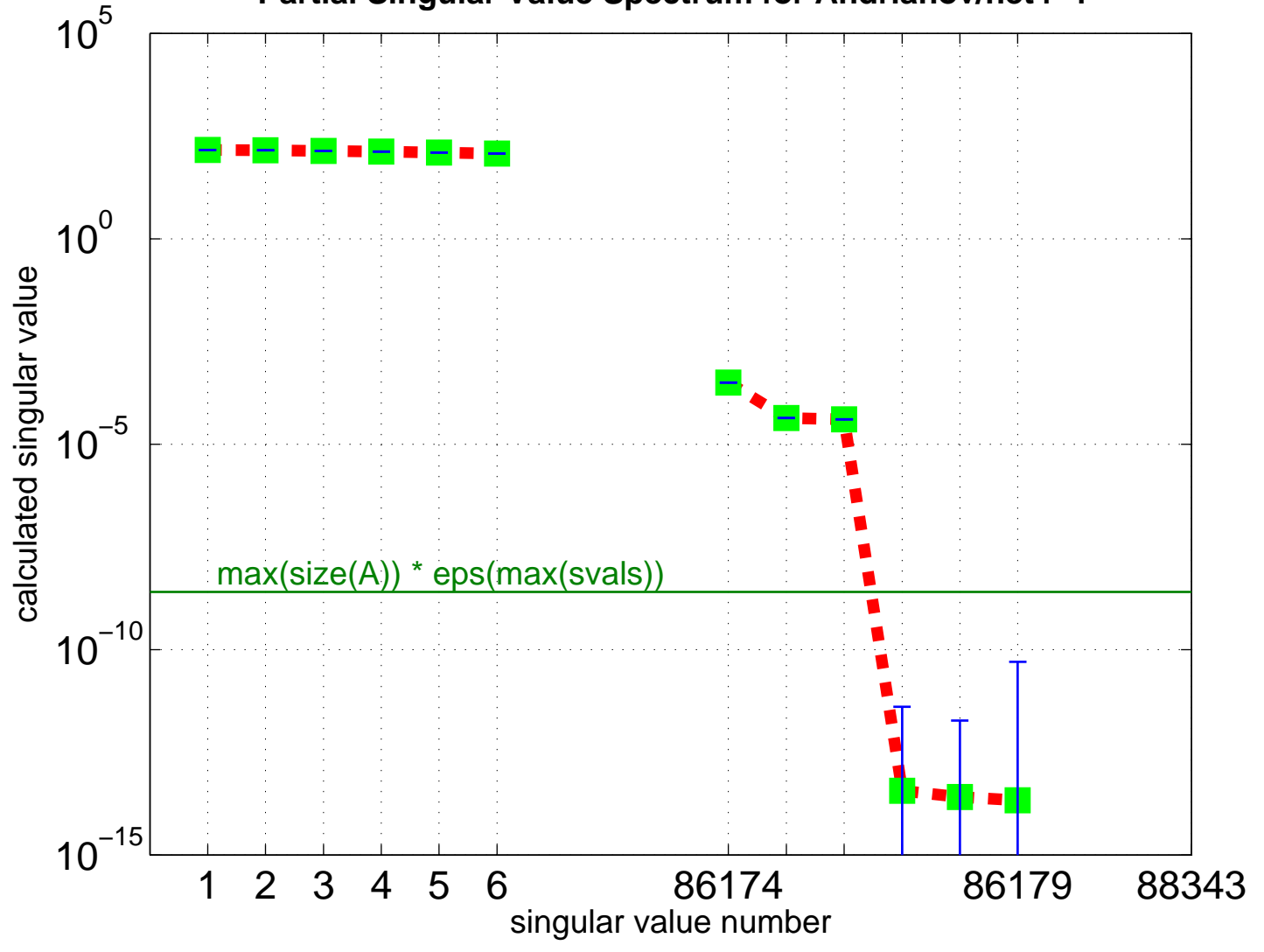
Partial Singular Value Spectrum for Andrianov/net4-1
