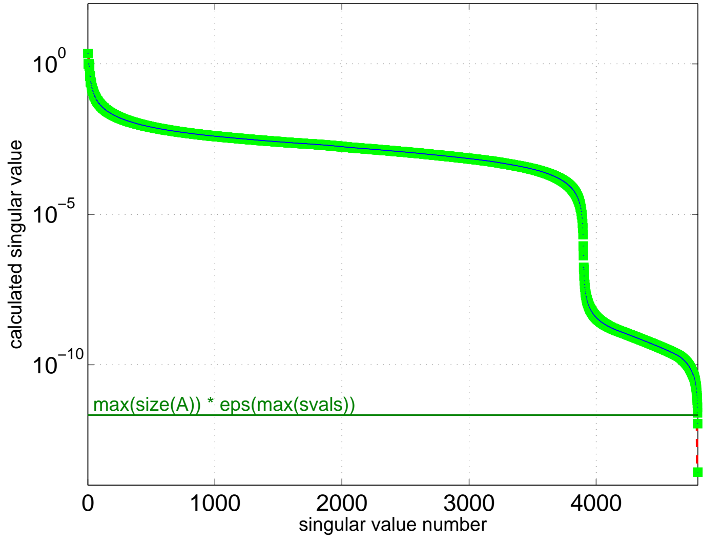
Singular Value Spectrum for Bai/mhd4800b
