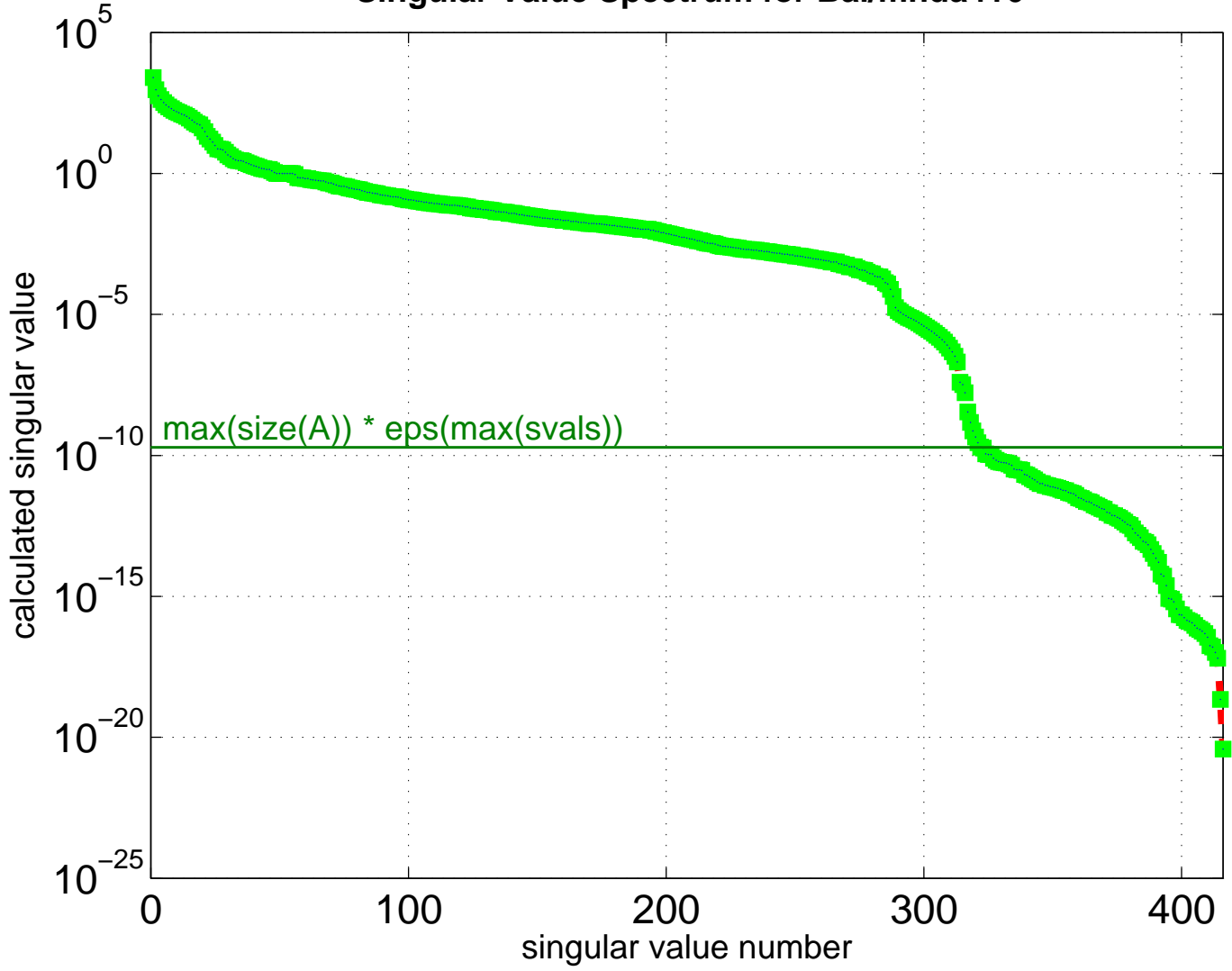
Singular Value Spectrum for Bai/mhda416
