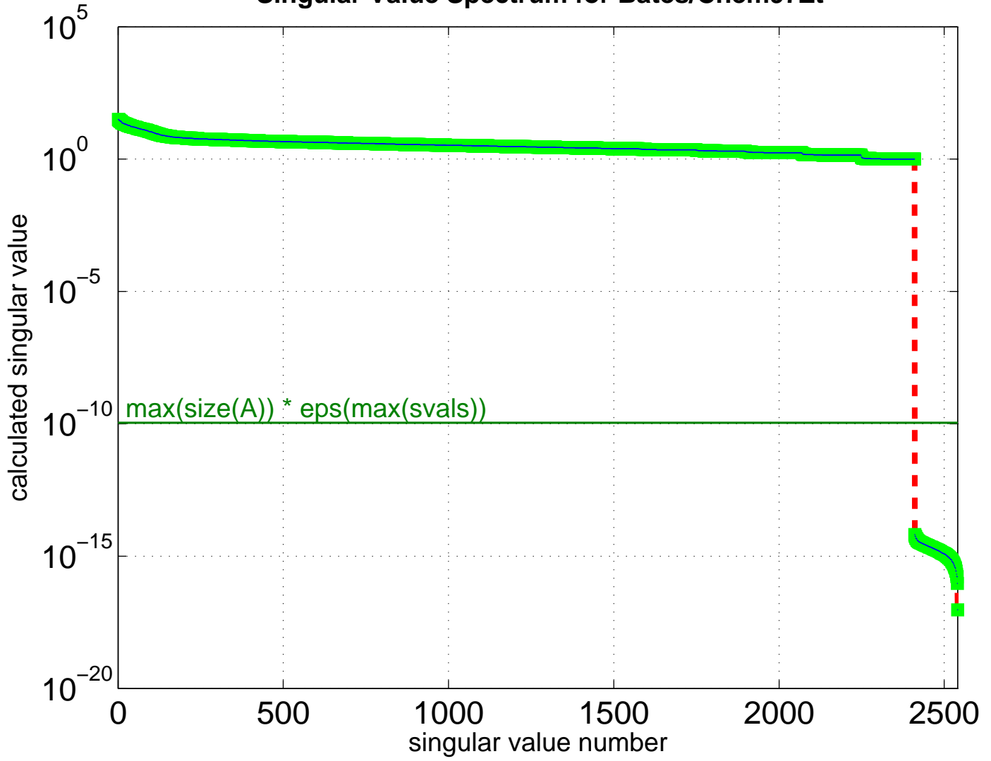
Singular Value Spectrum for Bates/Chem97Zt
