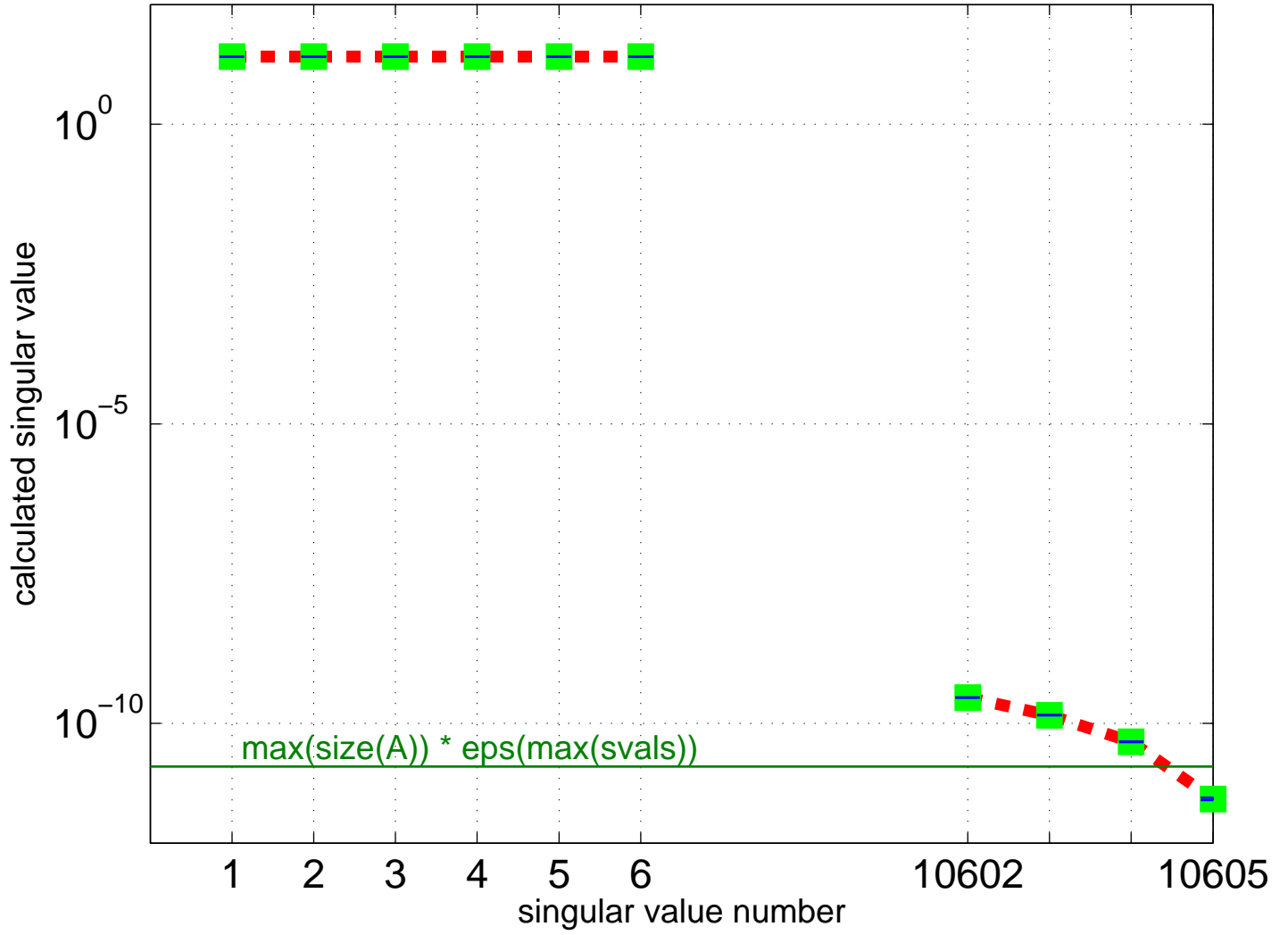
Partial Singular Value Spectrum for Bindel/ted_A
