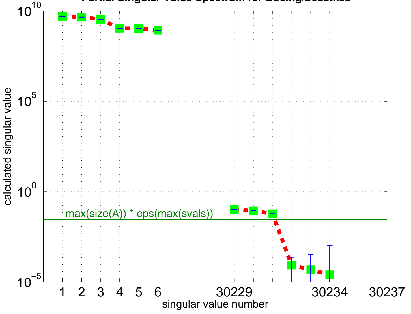
Partial Singular Value Spectrum for Boeing/bcsstk35
