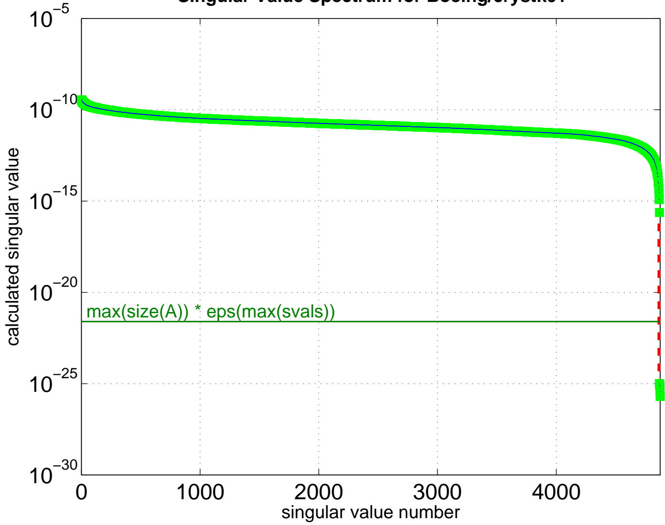
Singular Value Spectrum for Boeing/crystk01
