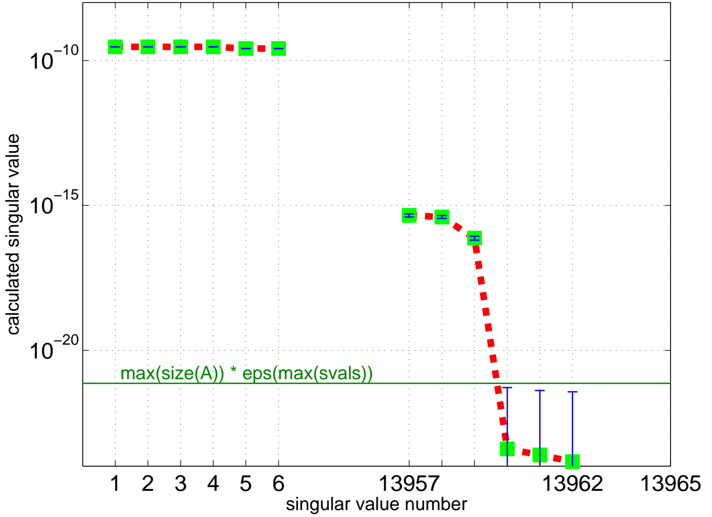
Partial Singular Value Spectrum for Boeing/crystk02
