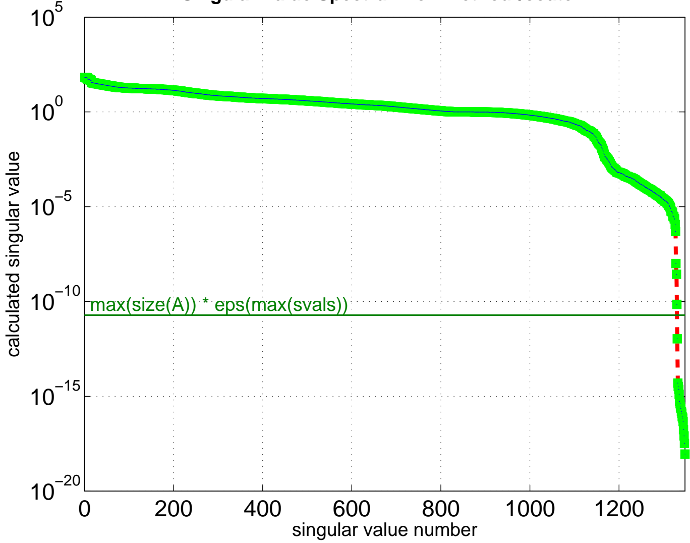
Singular Value Spectrum for Brethour/coater1
