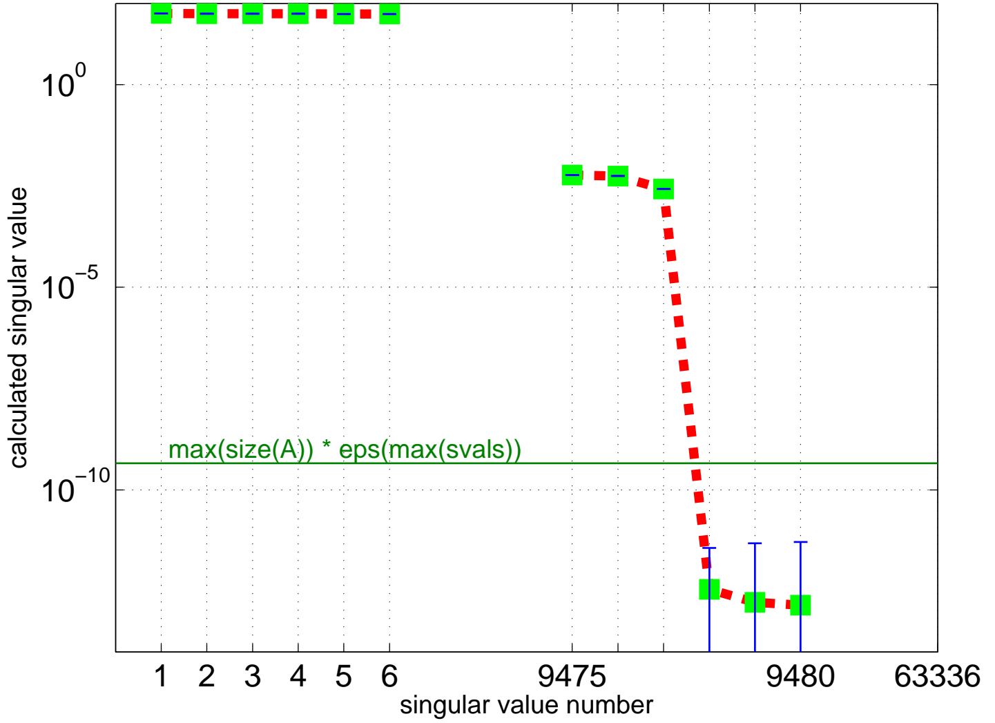
Partial Singular Value Spectrum for Chen/pkustk03
