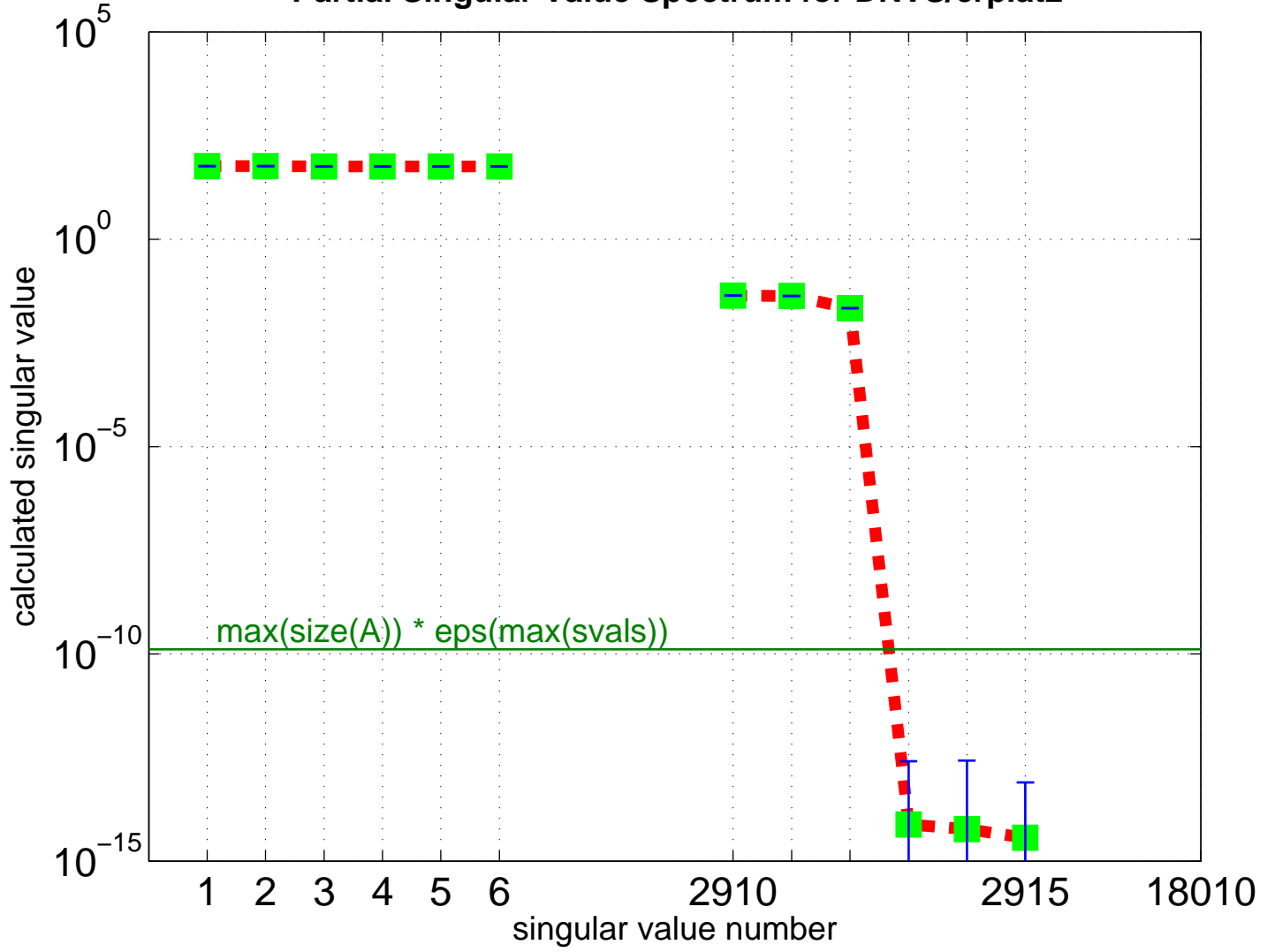
Partial Singular Value Spectrum for DNVs/crplat2
