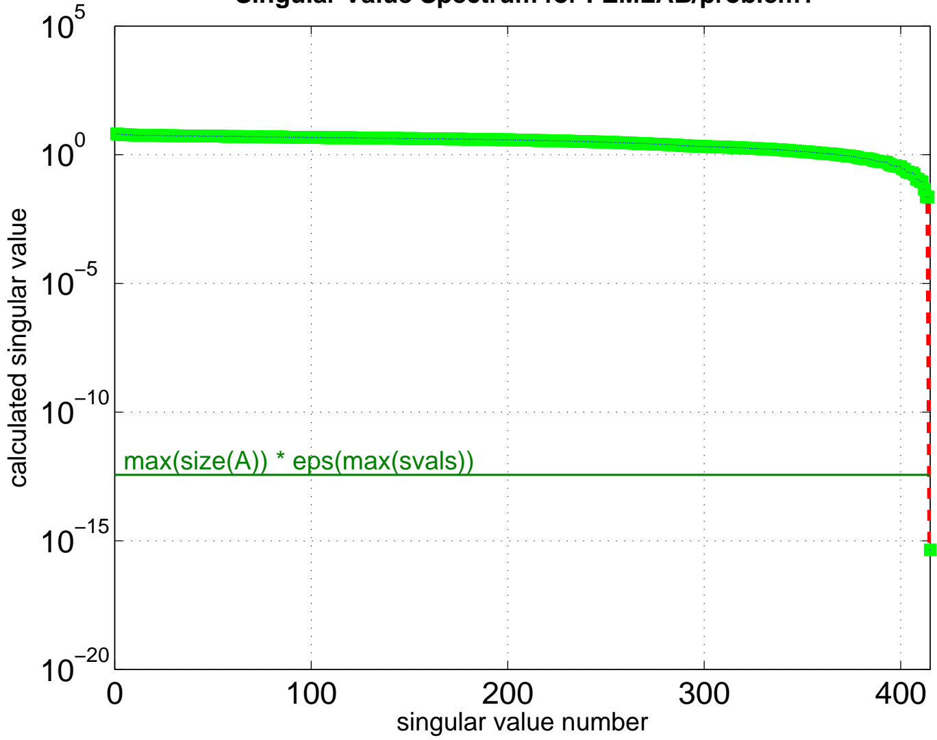
Singular Value Spectrum for FEMLAB/problem1
