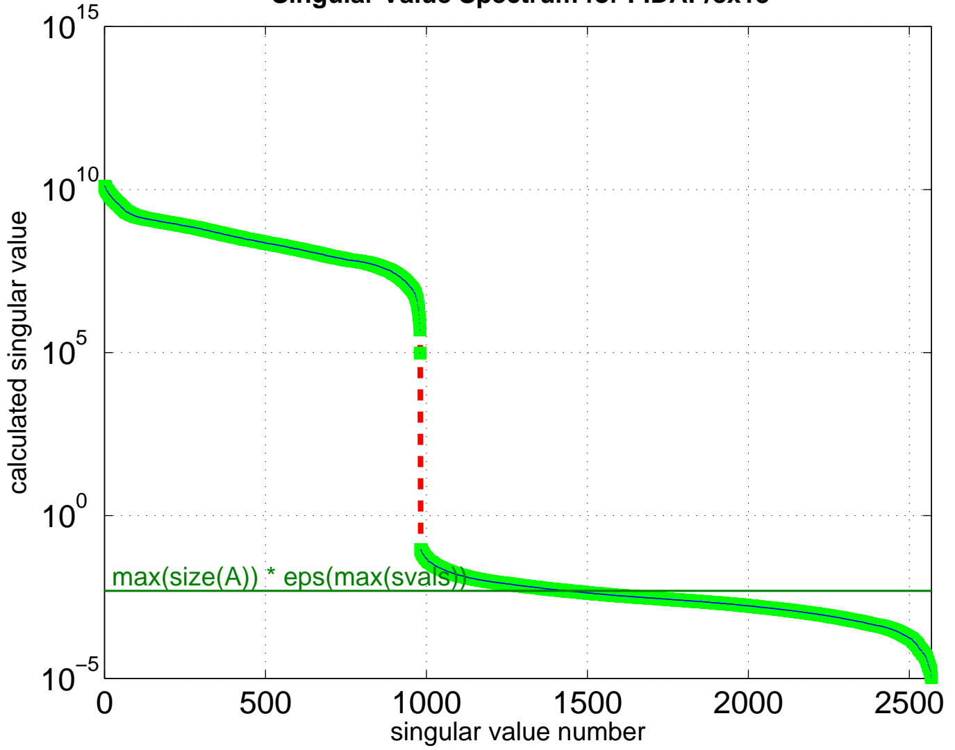
Singular Value Spectrum for FIDAP/ex13
