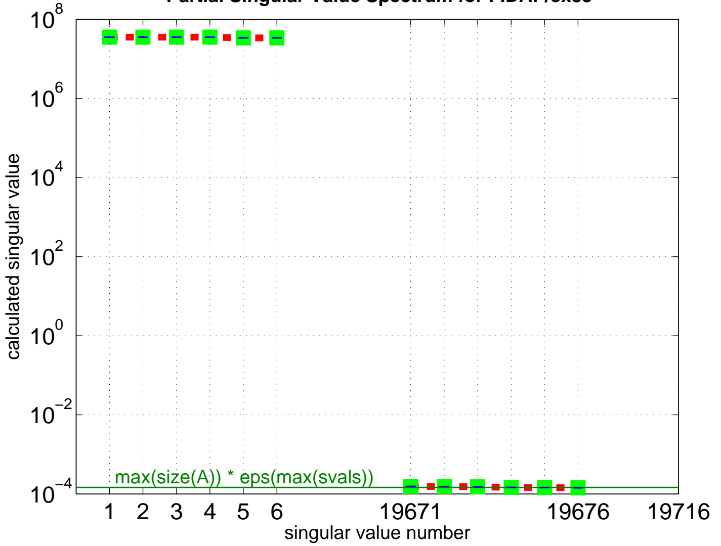
Partial Singular Value Spectrum for FIDAP/ex35
