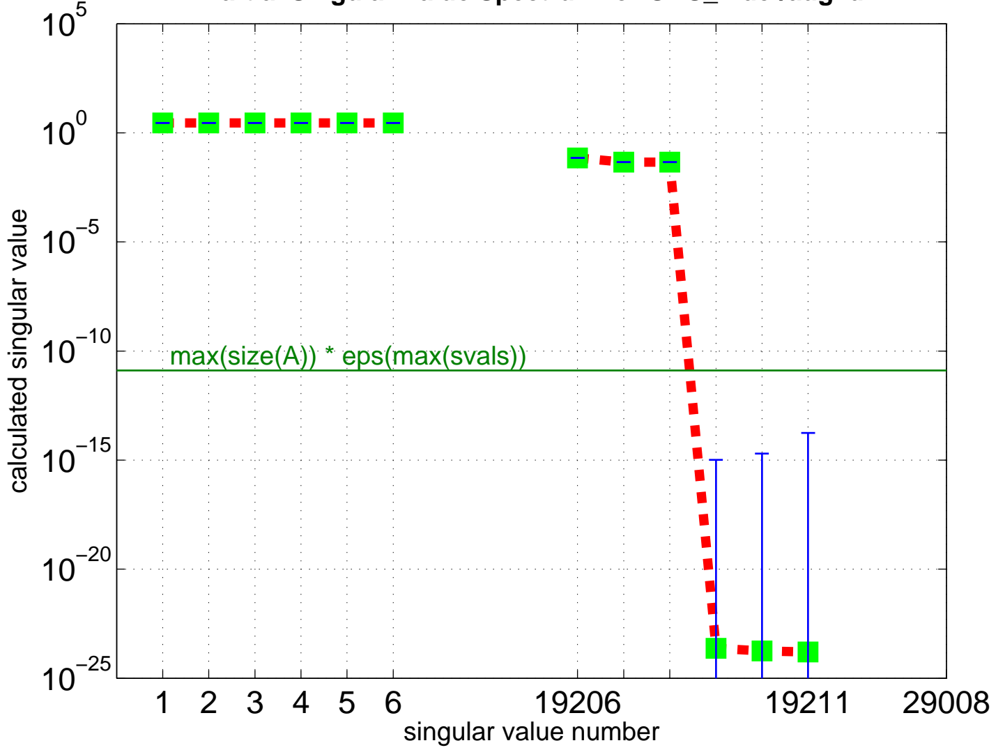
Partial Singular Value Spectrum for GHS_indef/aug2d
