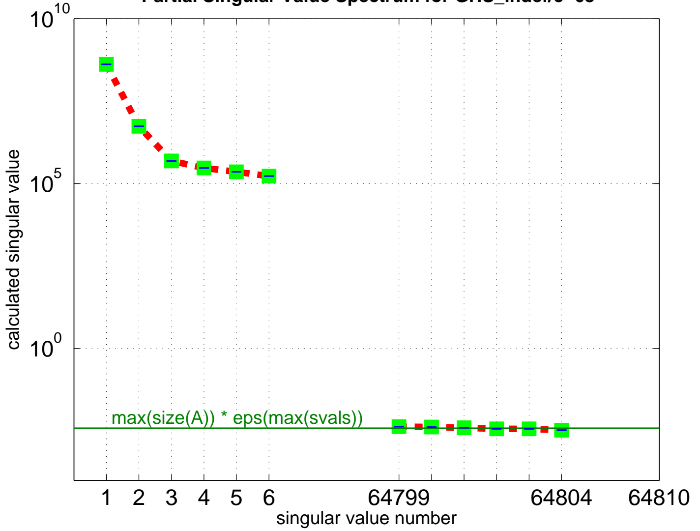
Partial Singular Value Spectrum for GHS_indef/c-68
