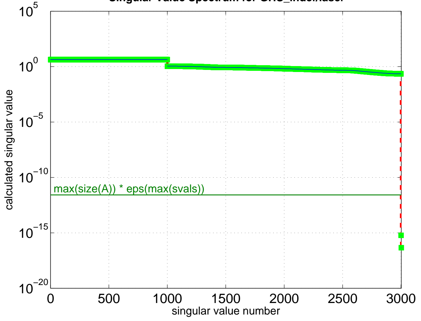
Singular Value Spectrum for GHS_indef/laser
