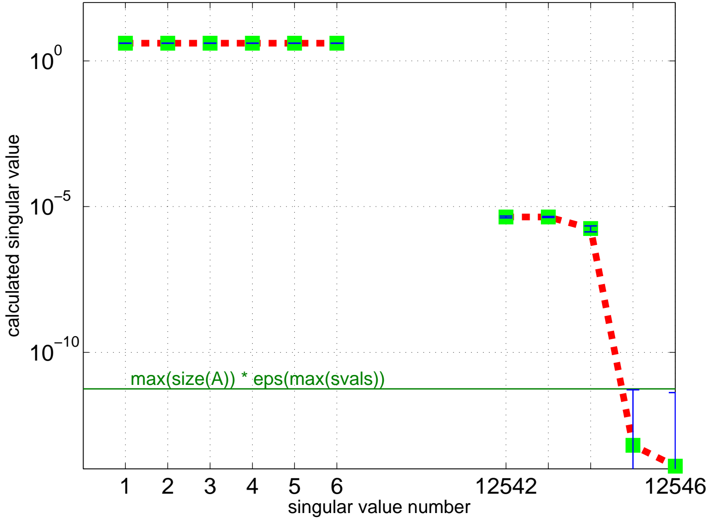
Partial Singular Value Spectrum for GHS_indef/stokes64
