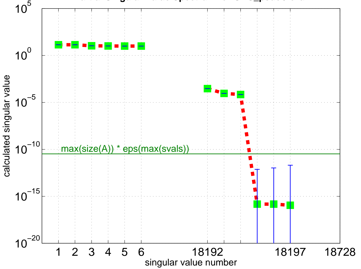
Partial Singular Value Spectrum for GHS_psdef/ford1
