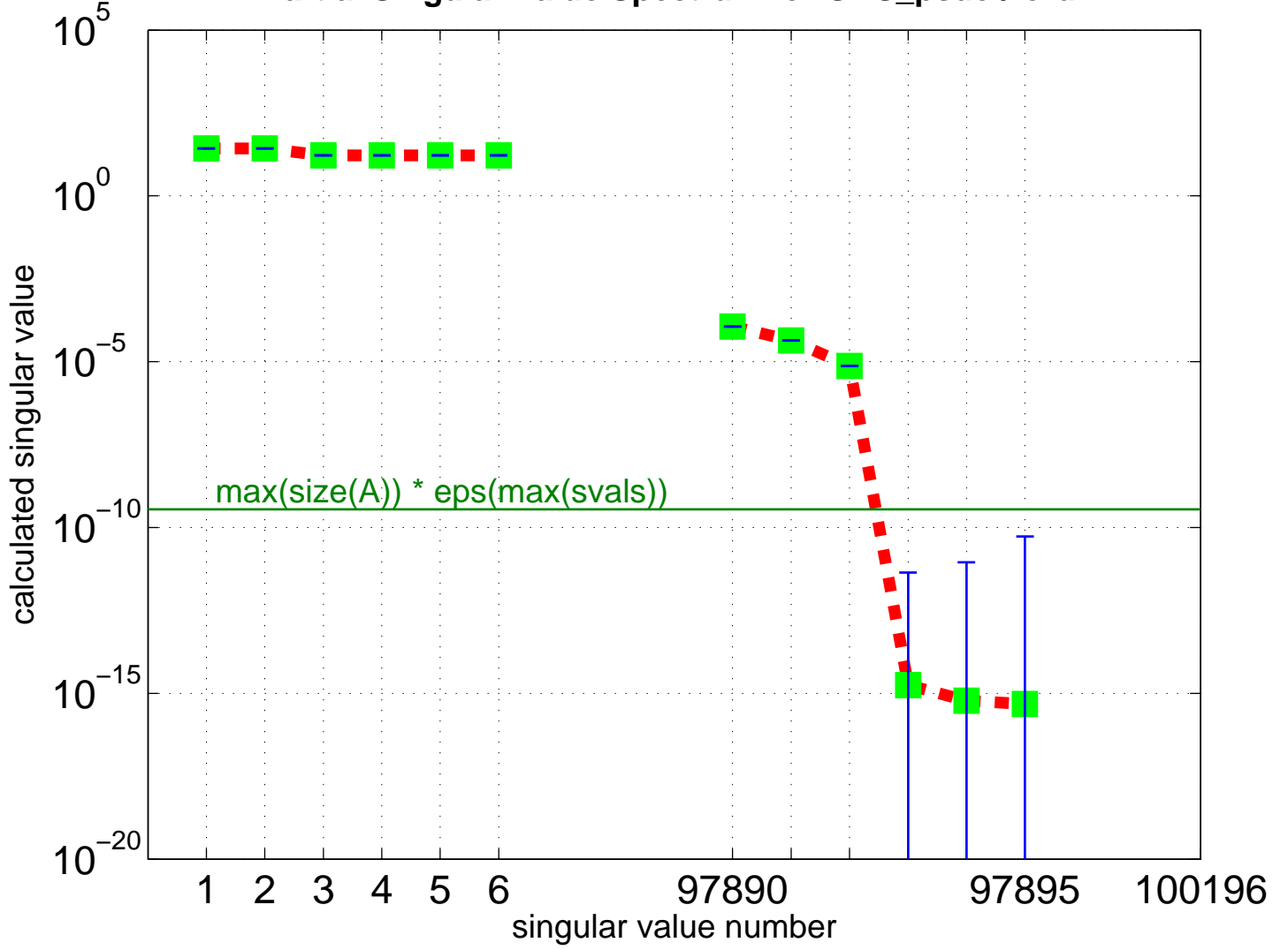
Partial Singular Value Spectrum for GHS_psdef/ford2
