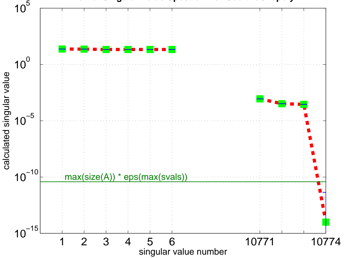
Partial Singular Value Spectrum for Gaertner/nopoly
