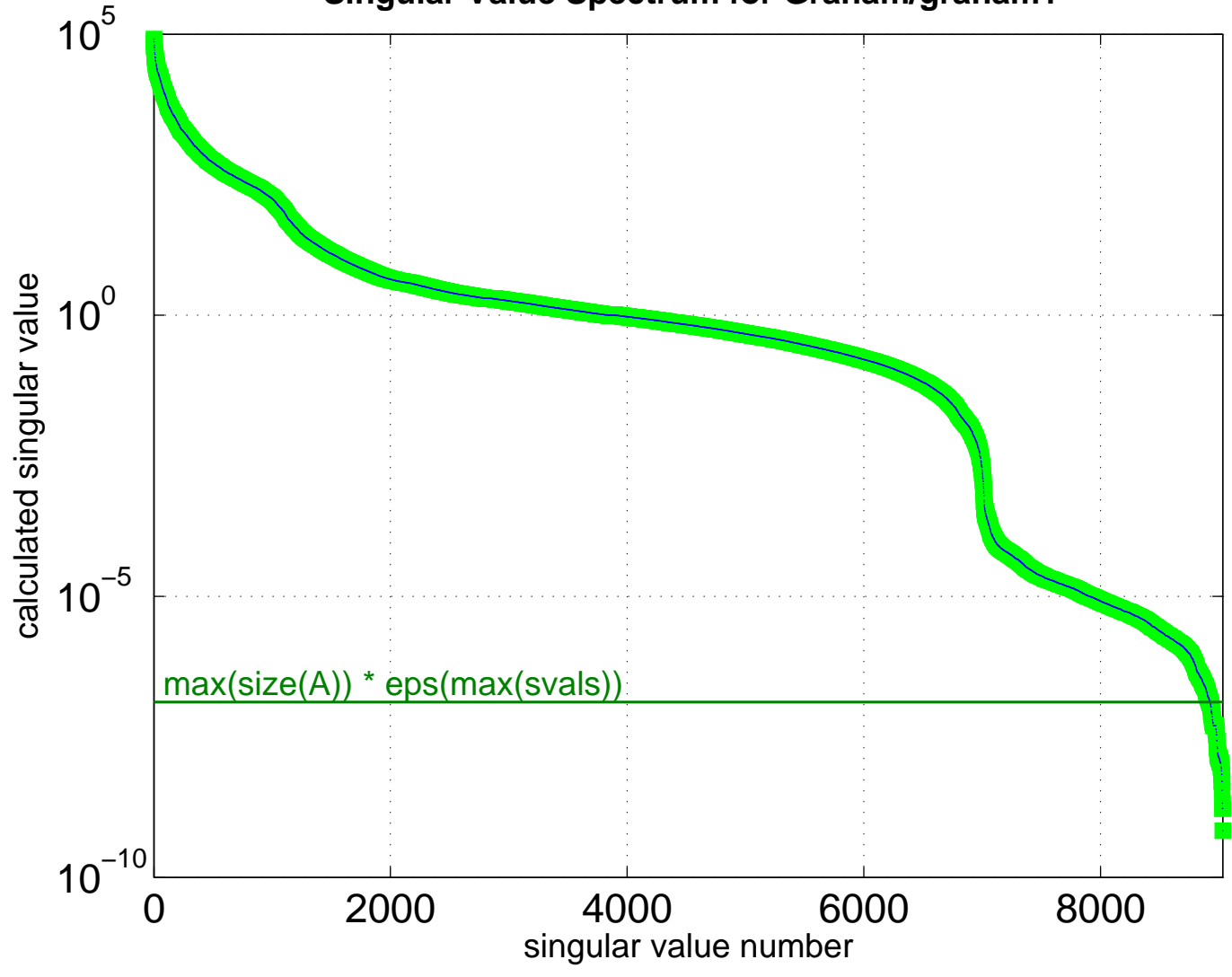
Singular Value Spectrum for Graham/graham1
