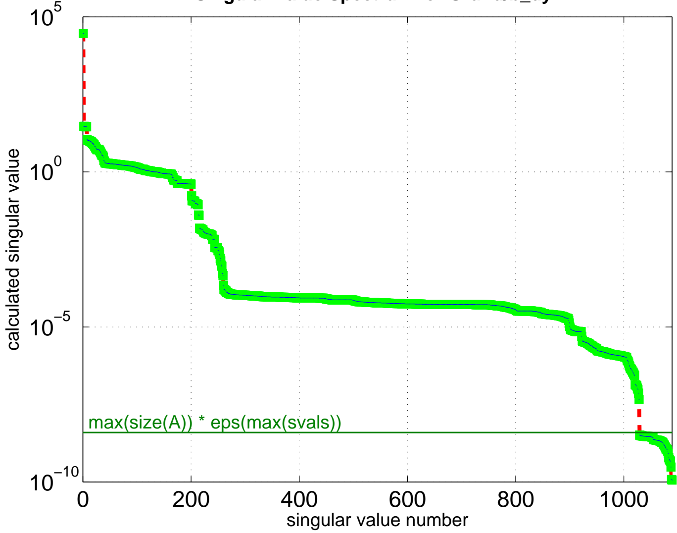
Singular Value Spectrum for Grund/b_dyn
