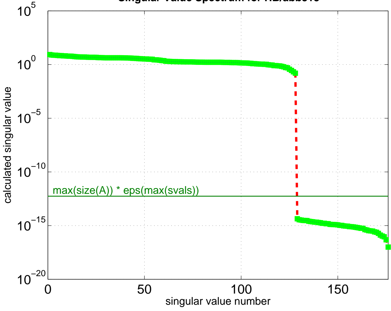
Singular Value Spectrum for HB/abb313
