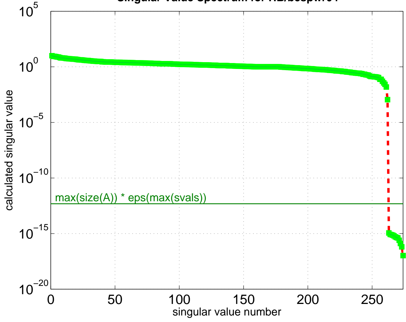
Singular Value Spectrum for HB/bcspwr04
