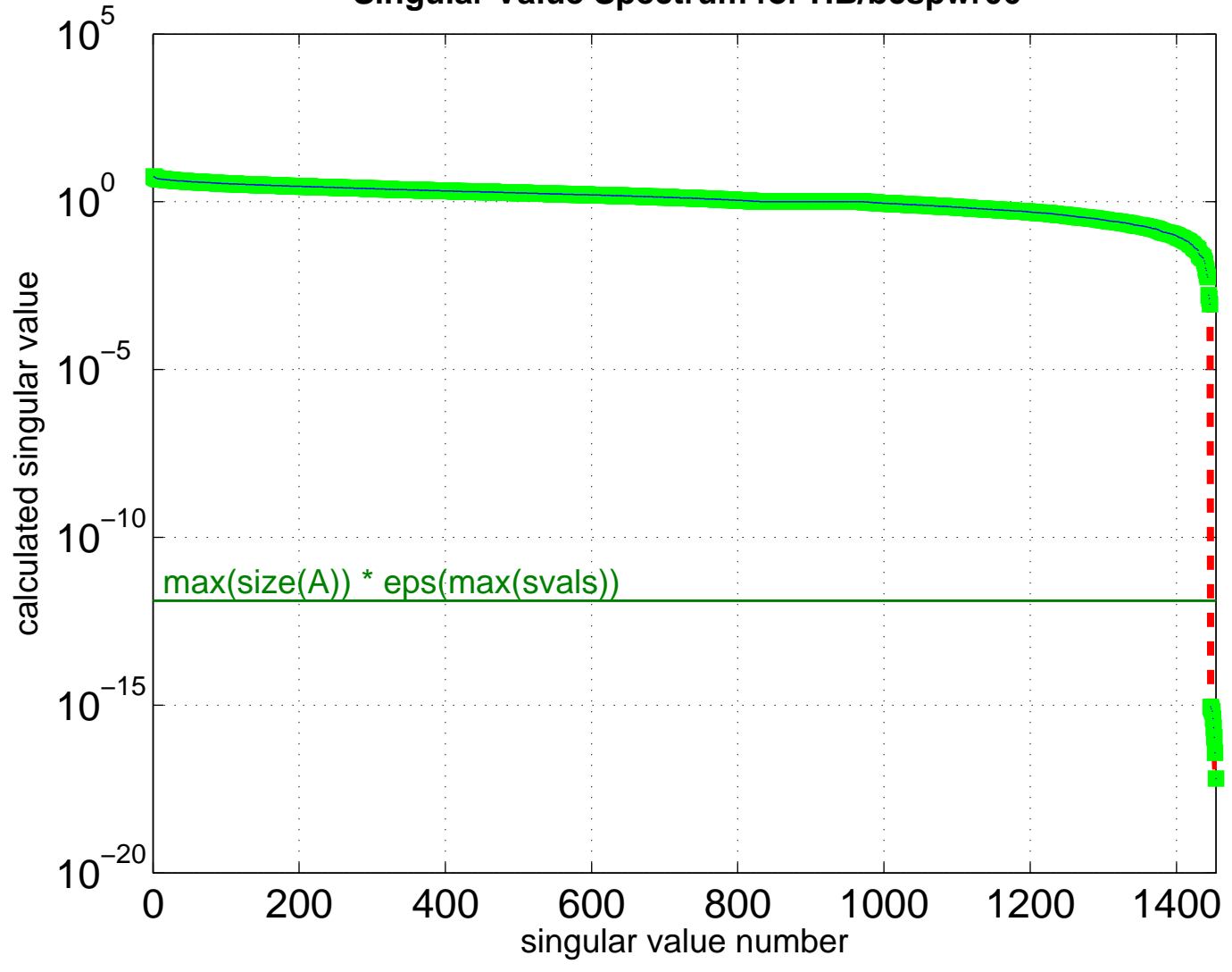
Singular Value Spectrum for HB/bcspwr06
