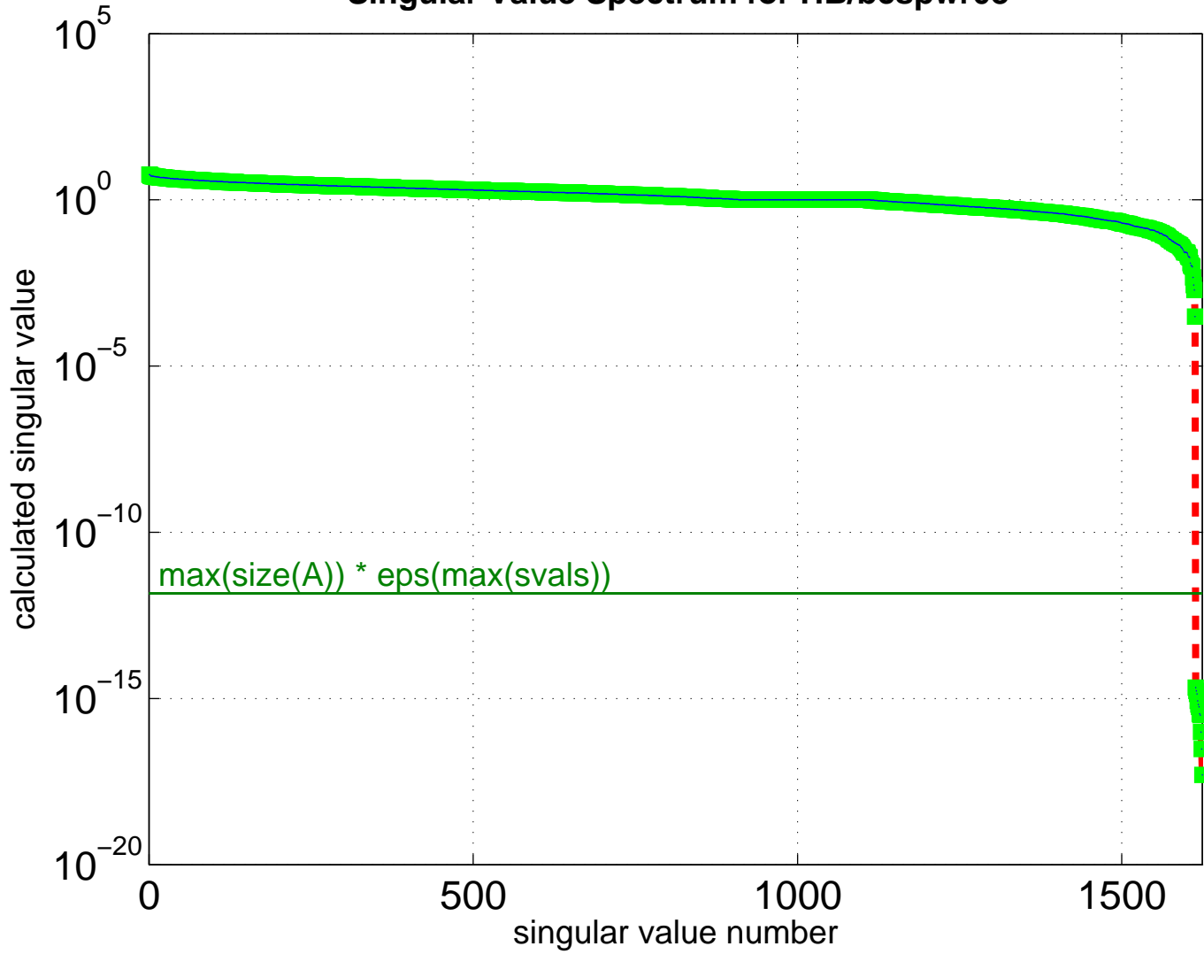
Singular Value Spectrum for HB/bcspwr08
