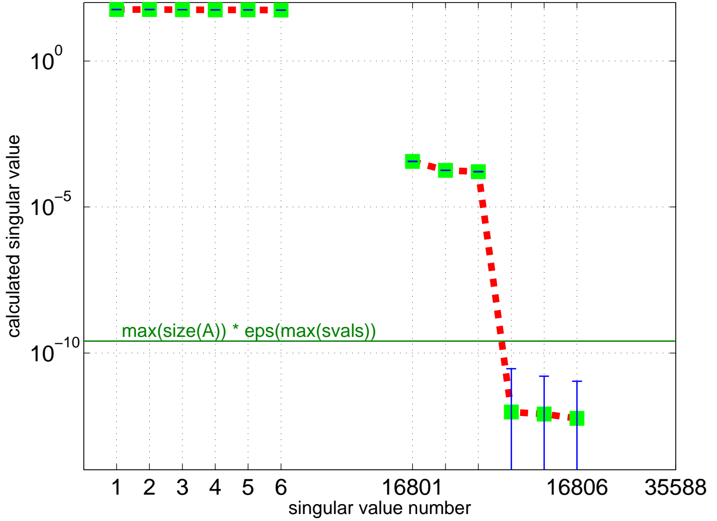
Partial Singular Value Spectrum for HB/bcsstk31
