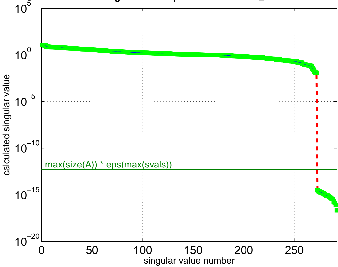
Singular Value Spectrum for HB/can_292
