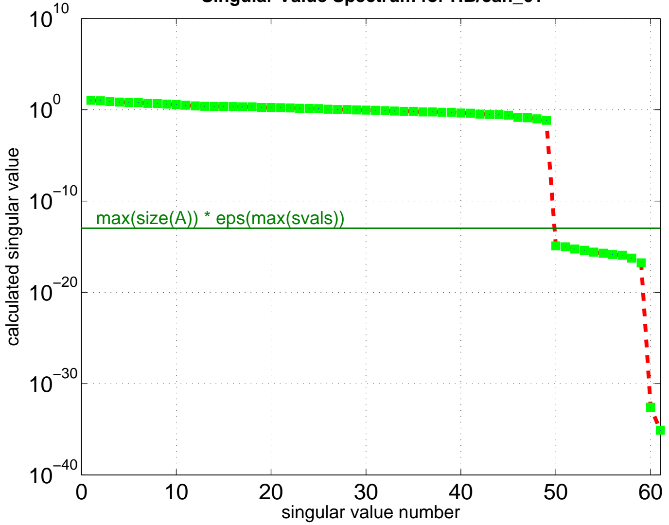
Singular Value Spectrum for HB/can_61
