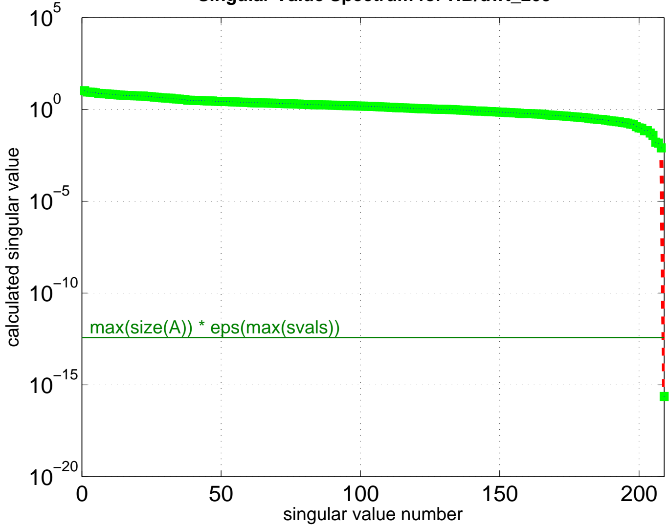
Singular Value Spectrum for HB/dwt_209
