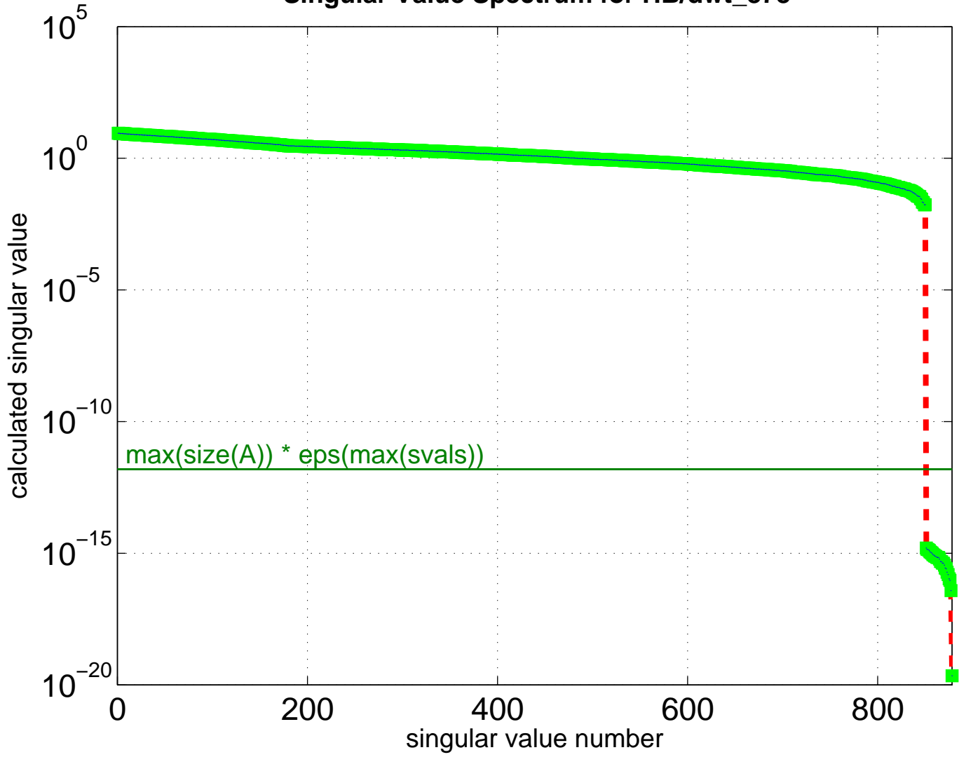
Singular Value Spectrum for HB/dwt_878
