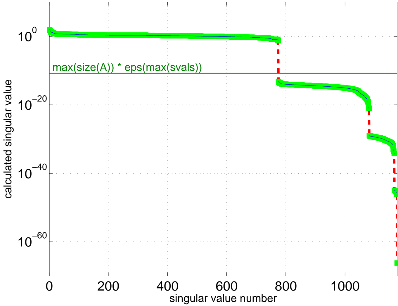
Singular Value Spectrum for HB/eris1176
