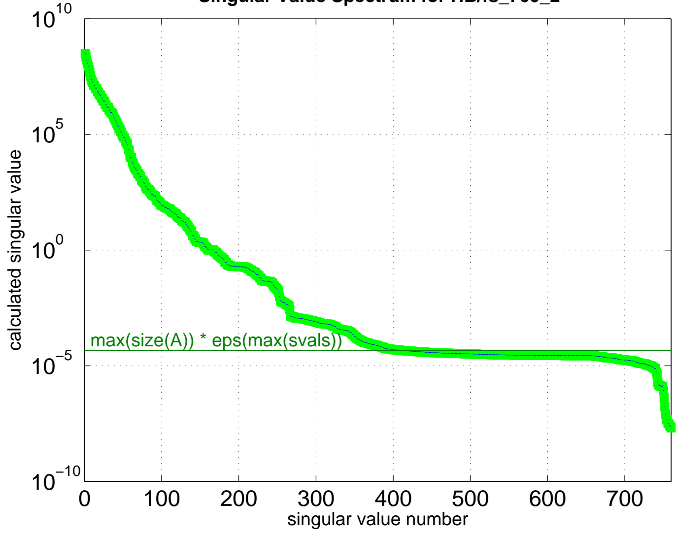
Singular Value Spectrum for HB/fs_760_2
