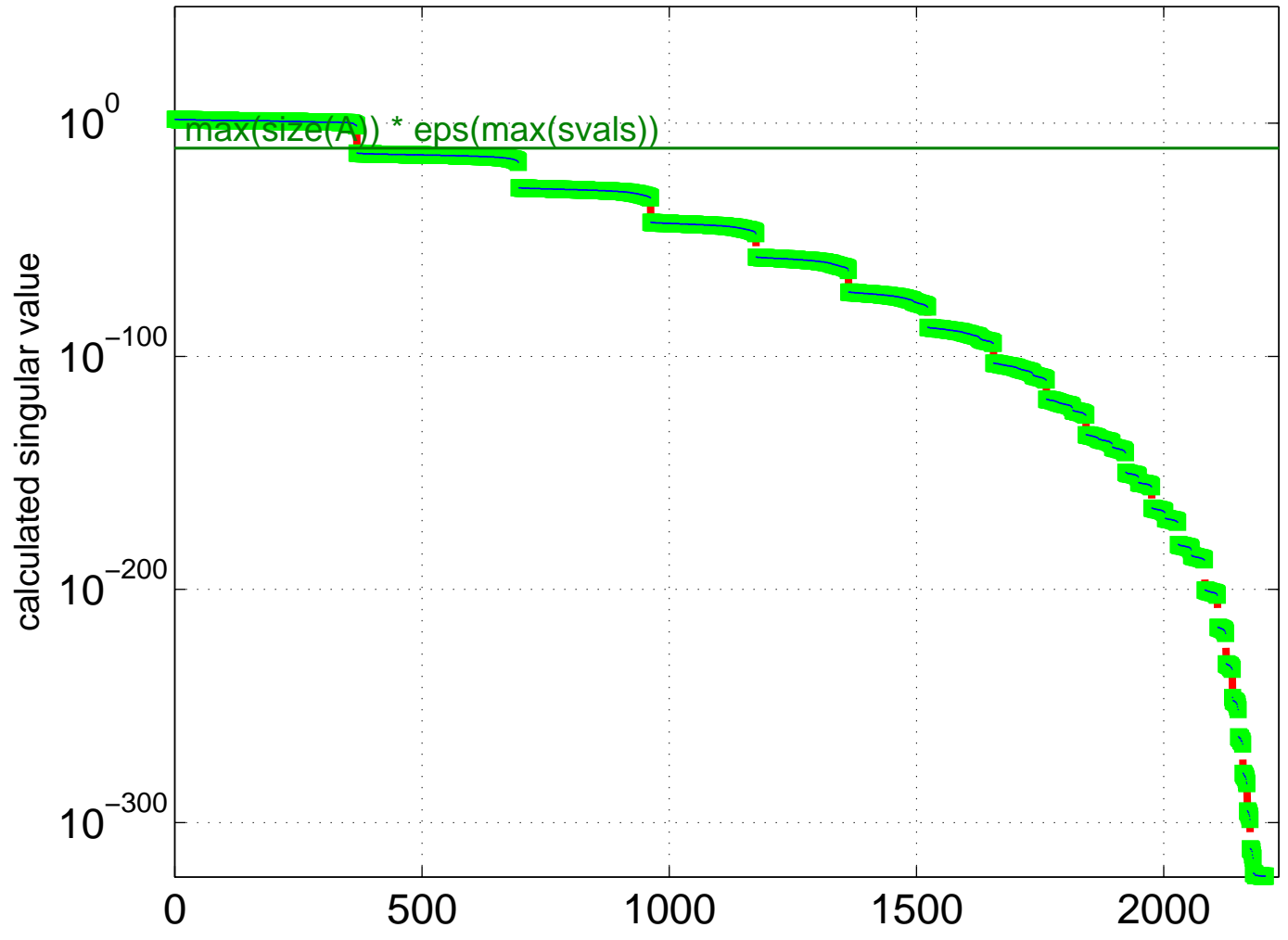
Singular Value Spectrum for HB/lock2232
