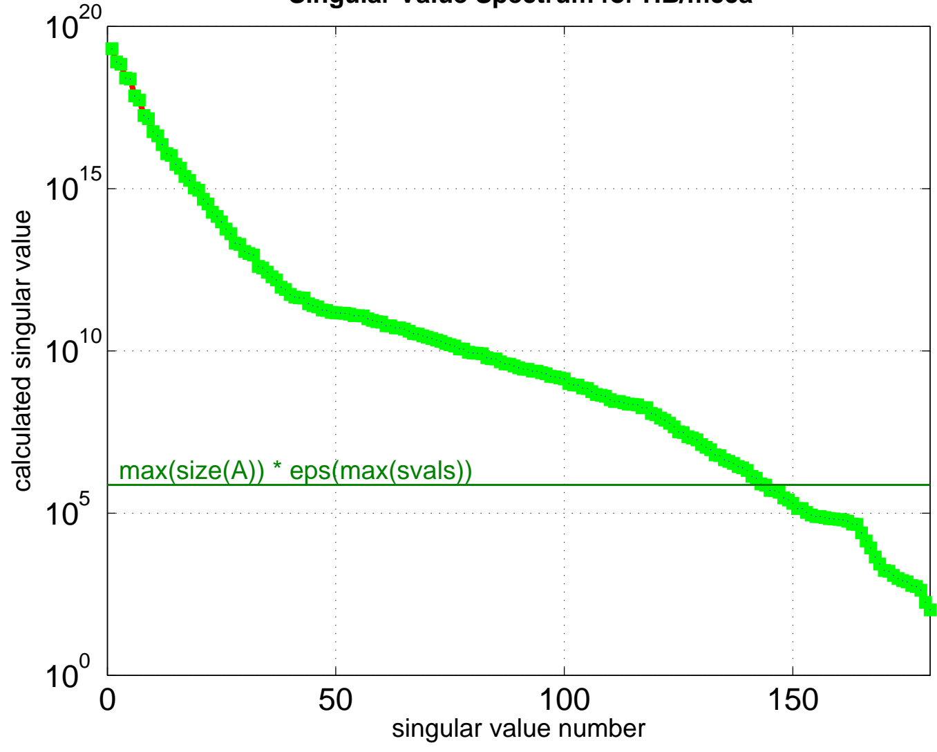
Singular Value Spectrum for HB/mcca
