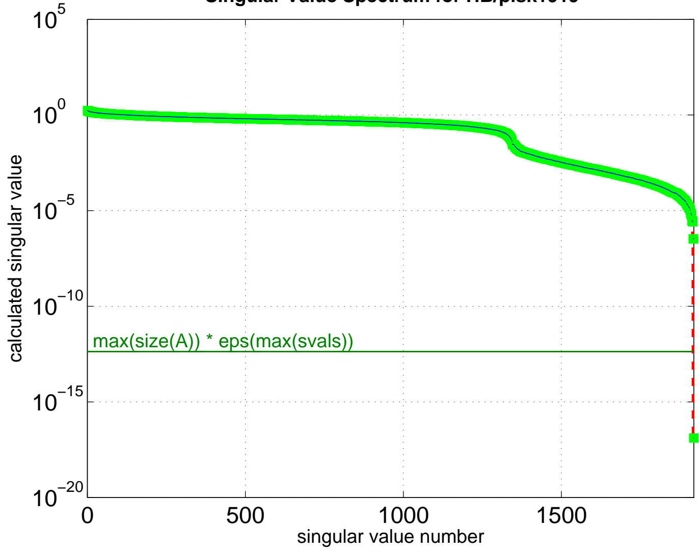
Singular Value Spectrum for HB/plsk1919
