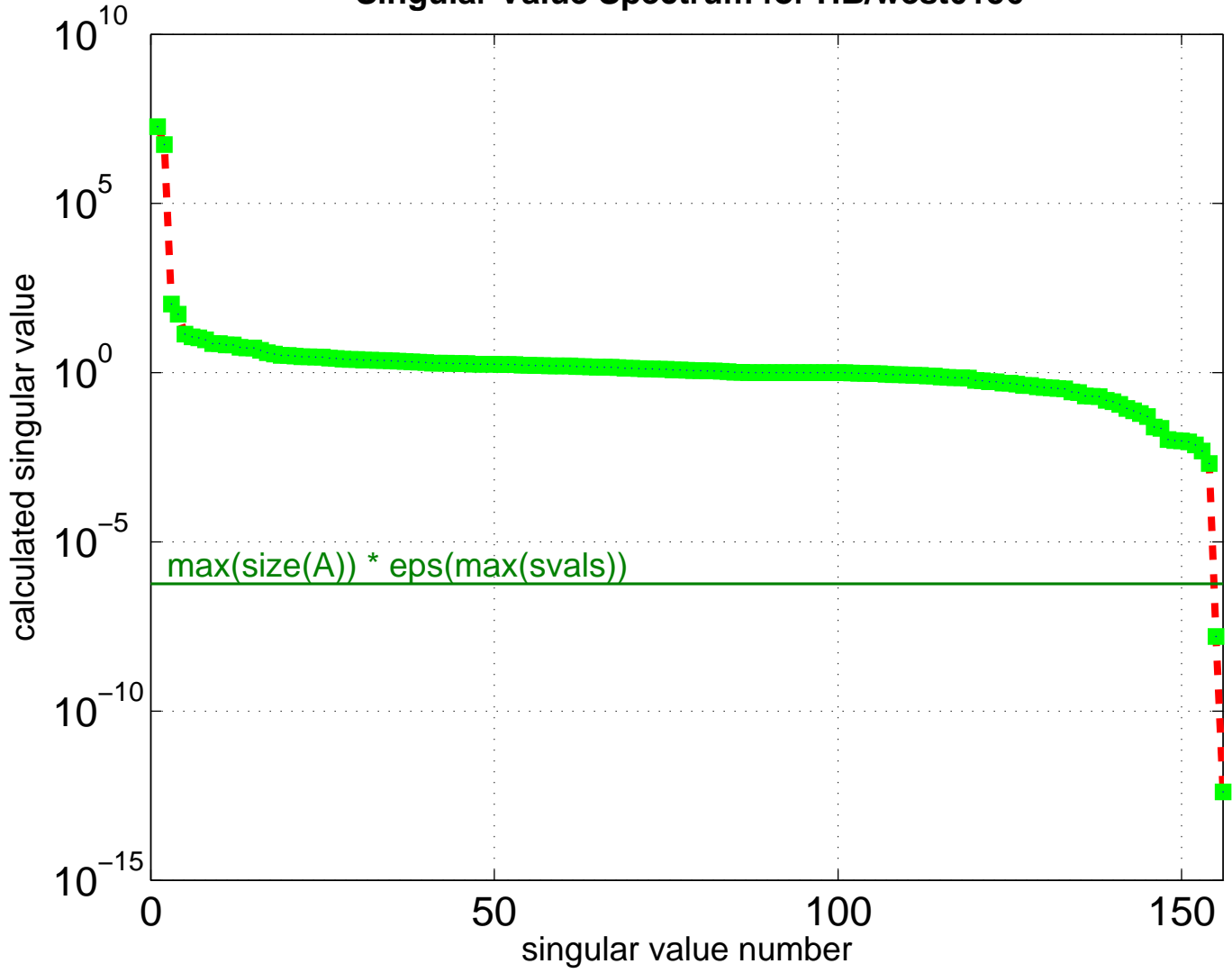
Singular Value Spectrum for HB/west0156
