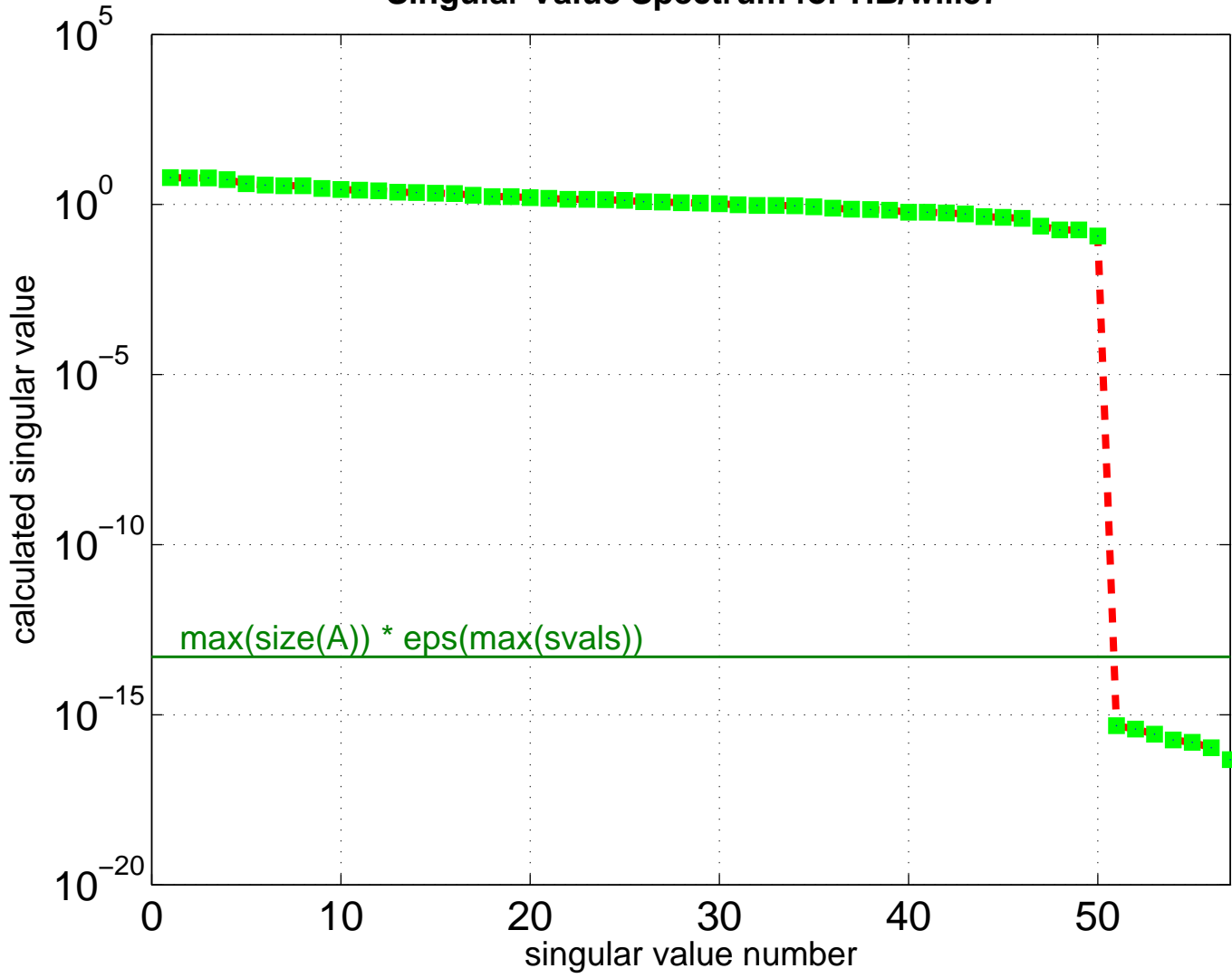
Singular Value Spectrum for HB/will57
