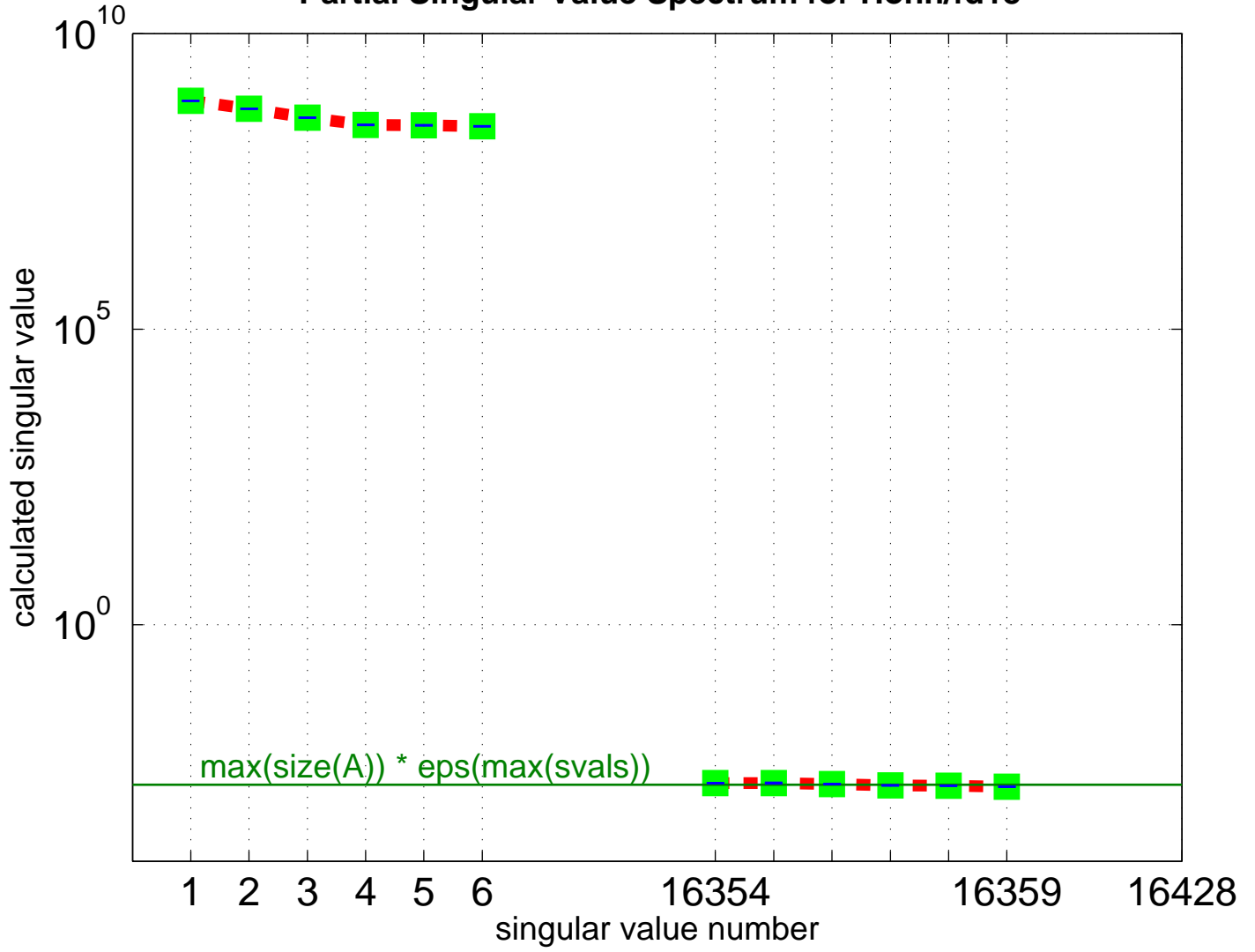
Partial Singular Value Spectrum for Hohn/fd18
