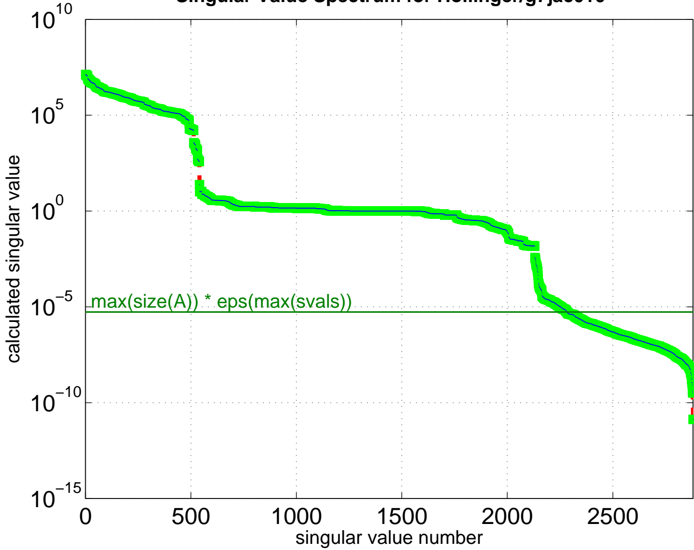
Singular Value Spectrum for Hollinger/g7jac010
