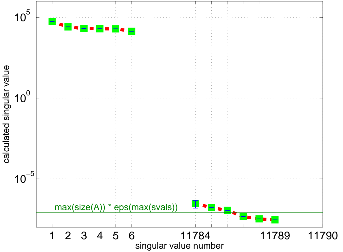
Partial Singular Value Spectrum for Hollinger/g7jac040sc
