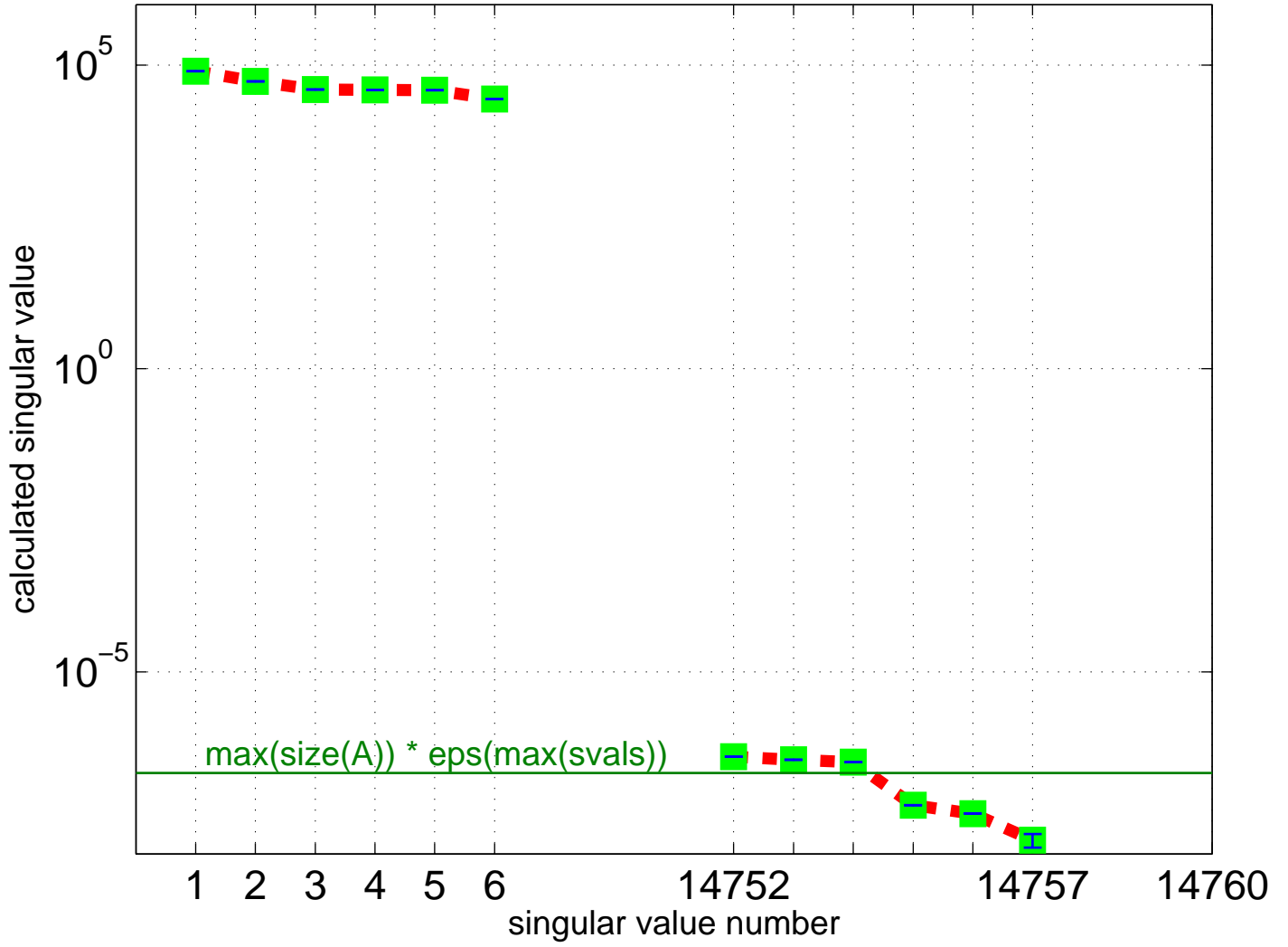
Partial Singular Value Spectrum for Hollinger/g7jac050sc
