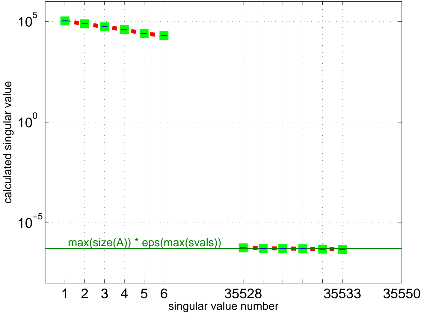
Partial Singular Value Spectrum for Hollinger/g7jac120sc
