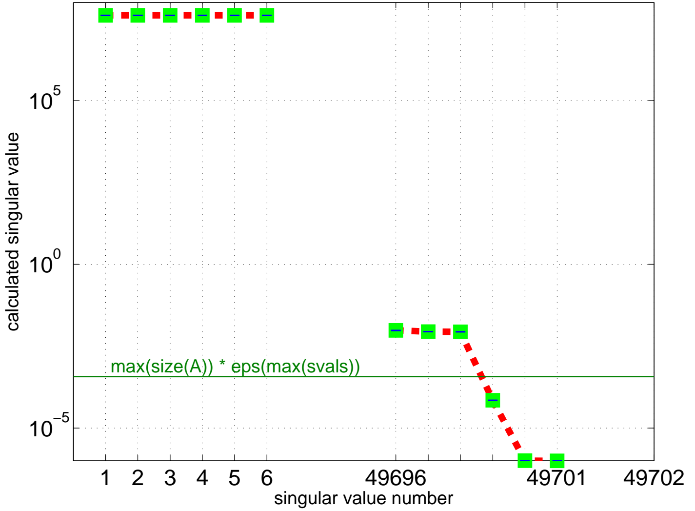
Partial Singular Value Spectrum for IBM_EDA/ckt11752_tr_0
