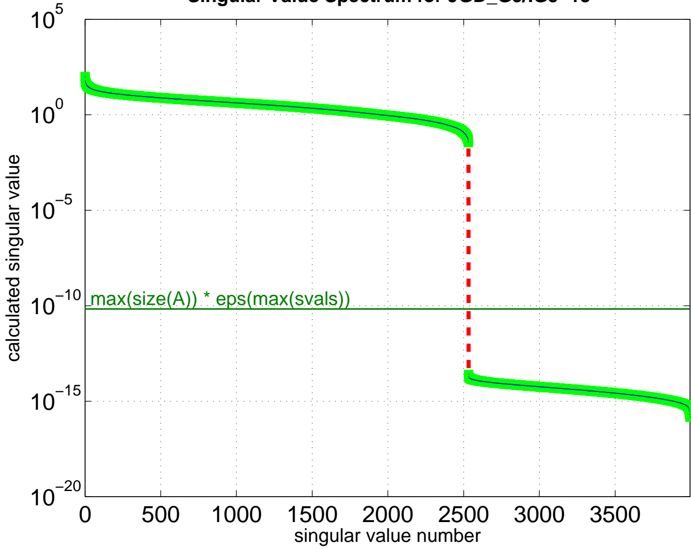
Singular Value Spectrum for JGD_G5/IG5-13
