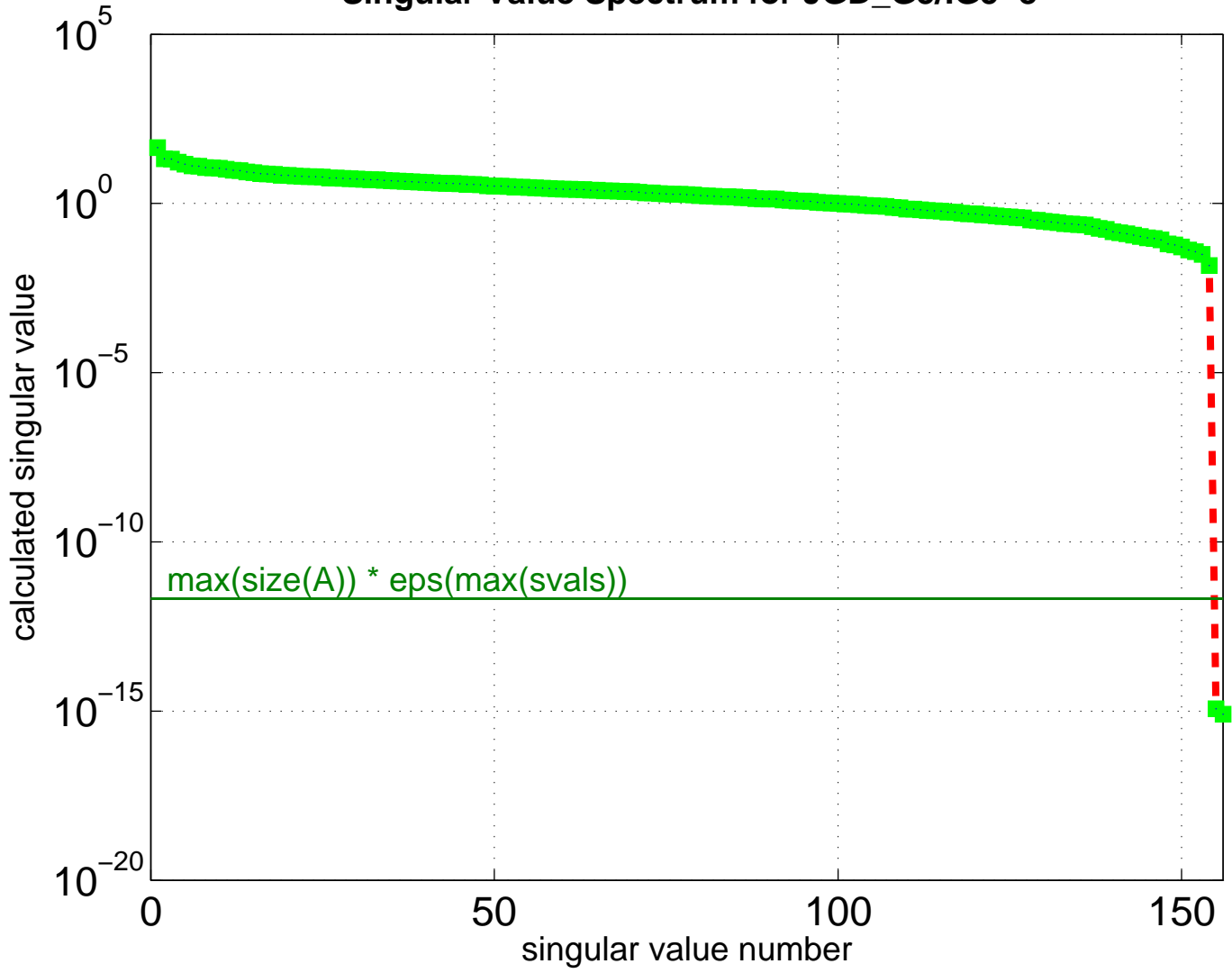
Singular Value Spectrum for JGD_G5/IG5-8
