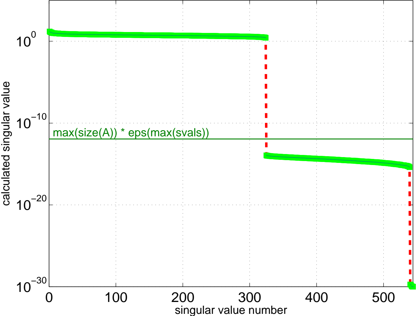
Singular Value Spectrum for JGD_GL6/GL6_D_8
