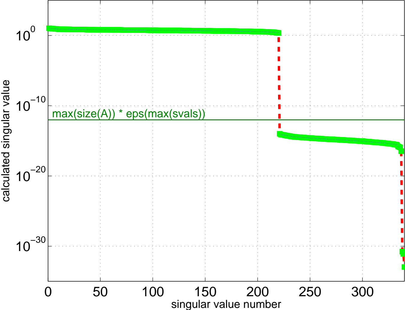
Singular Value Spectrum for JGD_GL6/GL6_D_9
