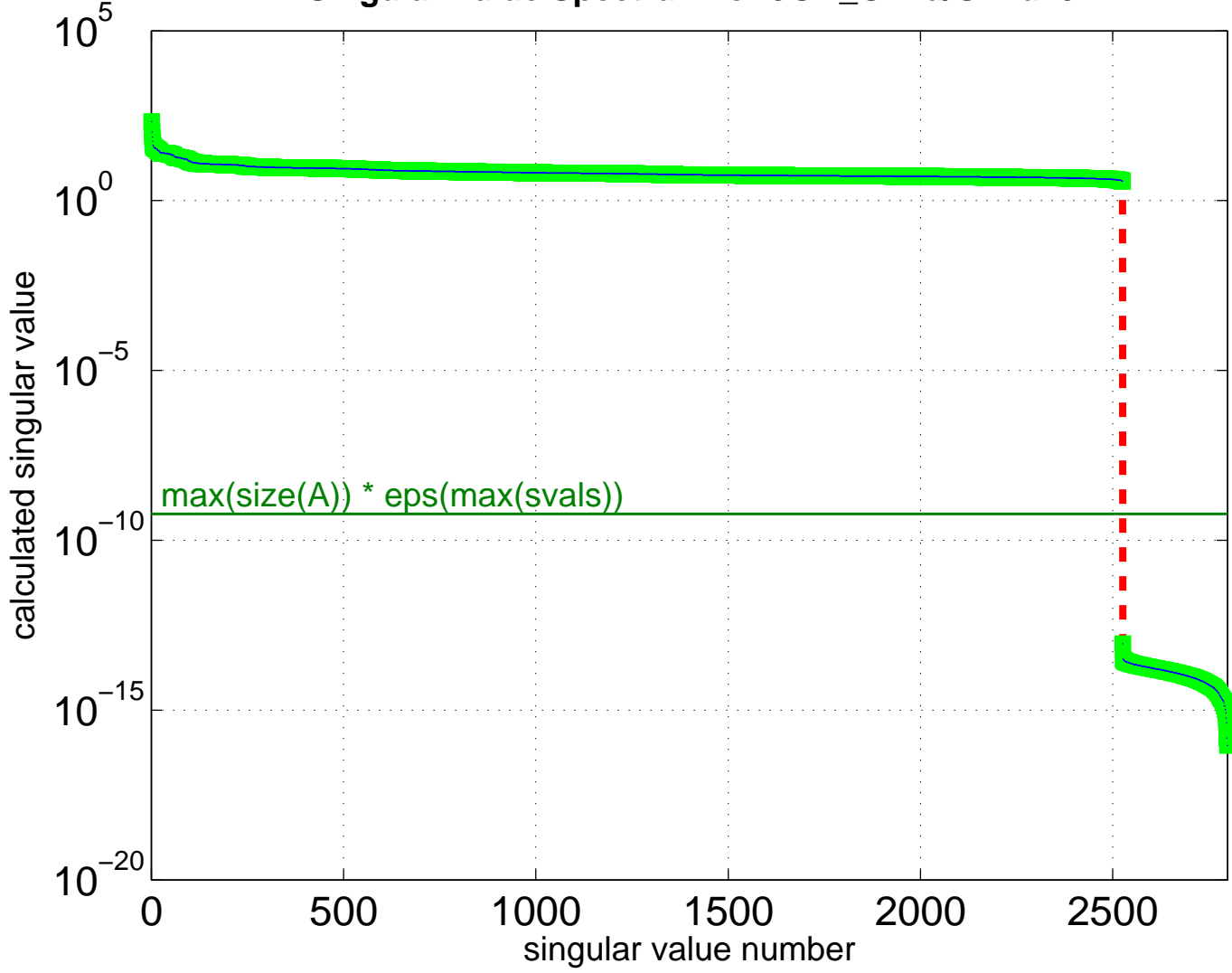
Singular Value Spectrum for JGD_GL7d/GL7d25
